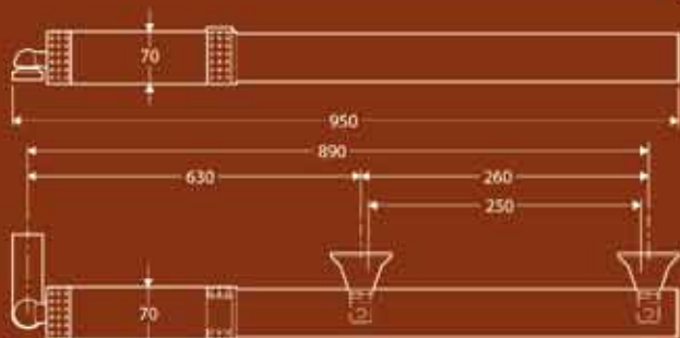
Swing Gates
